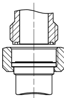
Rotalockanschluss Rotalock connection RLM / RLF
