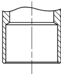
Rotalockanschluss Rotalock connection RLM / RLF
